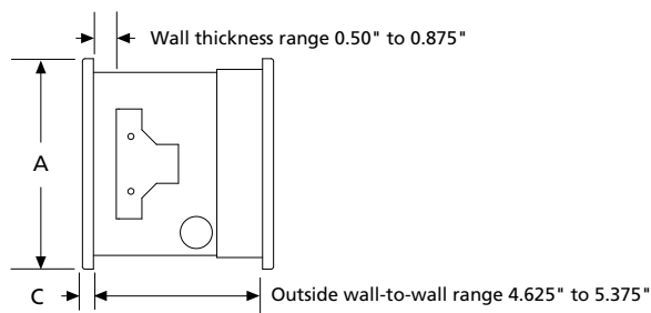
MSLT Side View
