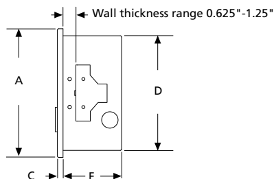
MSL/MSLD Side View
